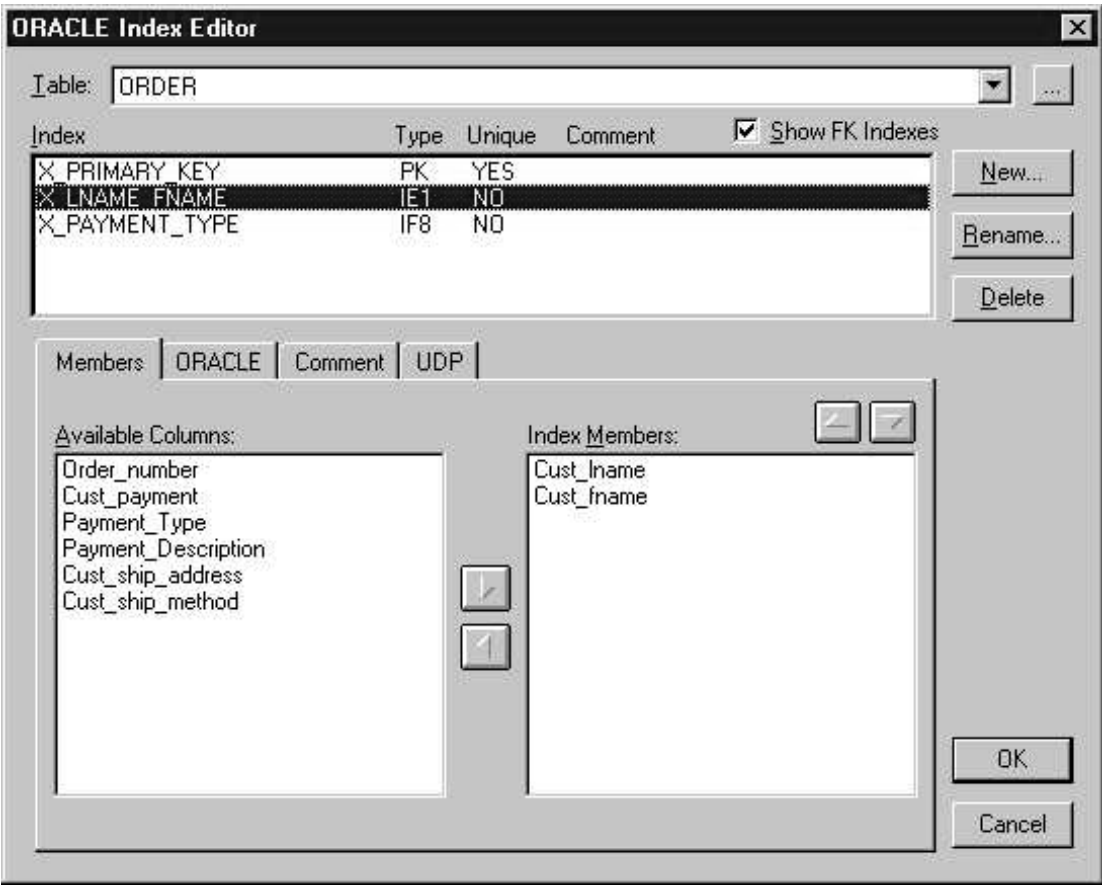
FIGURE 11-21 Indexes in ERwin
