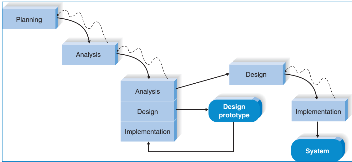
FIGURE 2-7 Throwaway Prototyping
