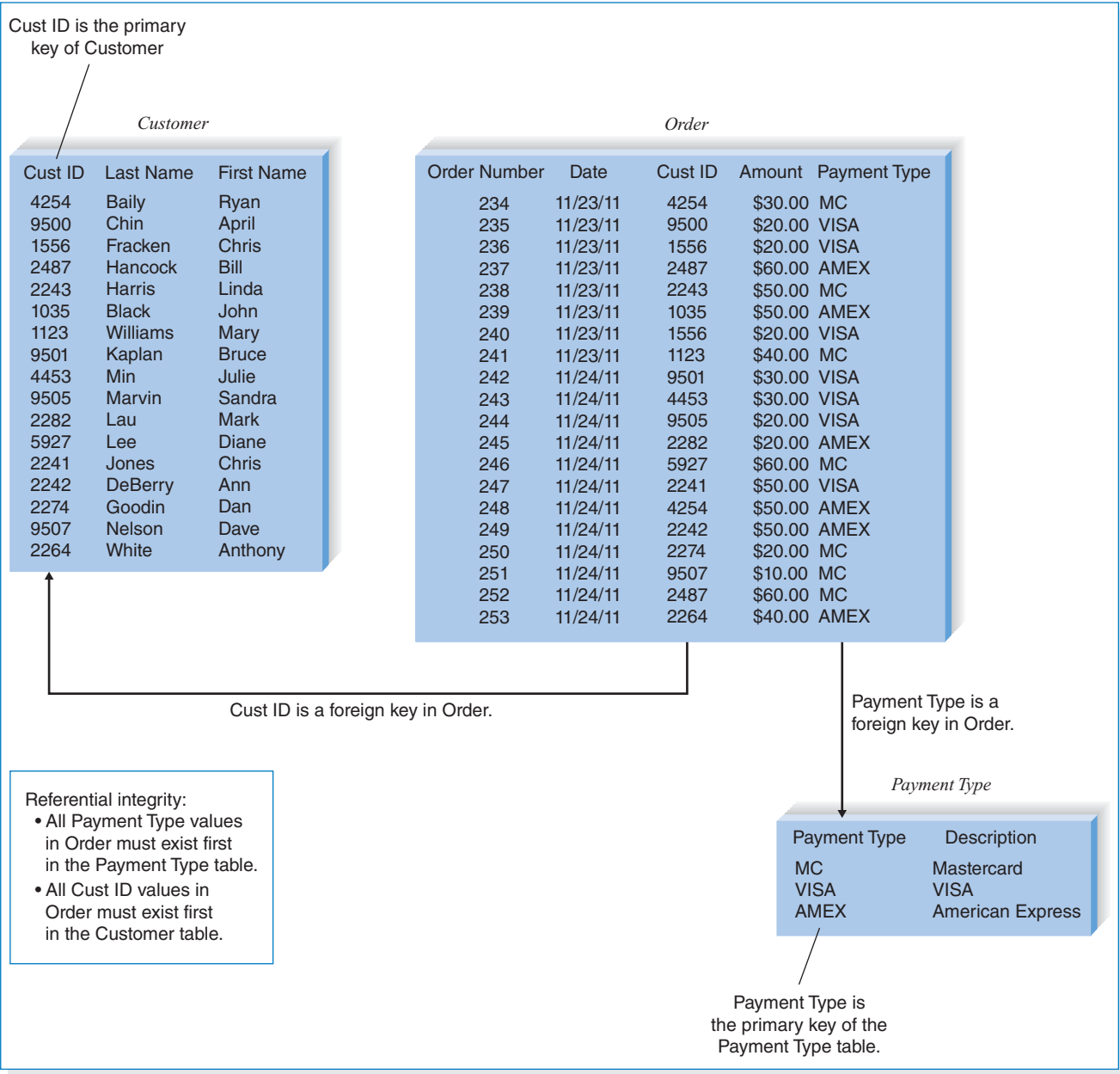
FIGURE 11-5 Relational Database
