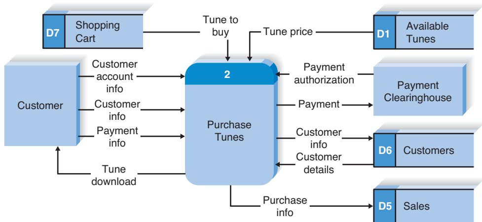
(b) Tune Source Process 2 DFD Fragment
