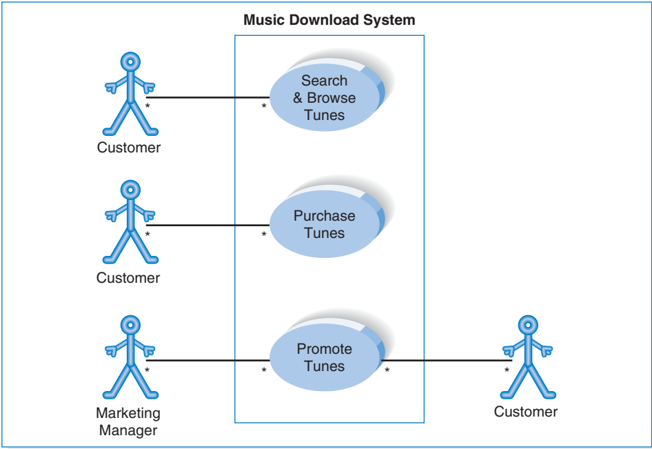
FIGURE 14-14 Tune Source Digital Music Download System Use Case Diagram
