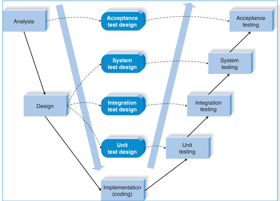
FIGURE 2-4 V-Model
