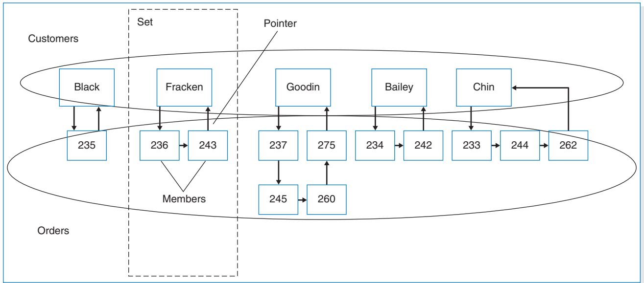
FIGURE 11-4 Network Database
