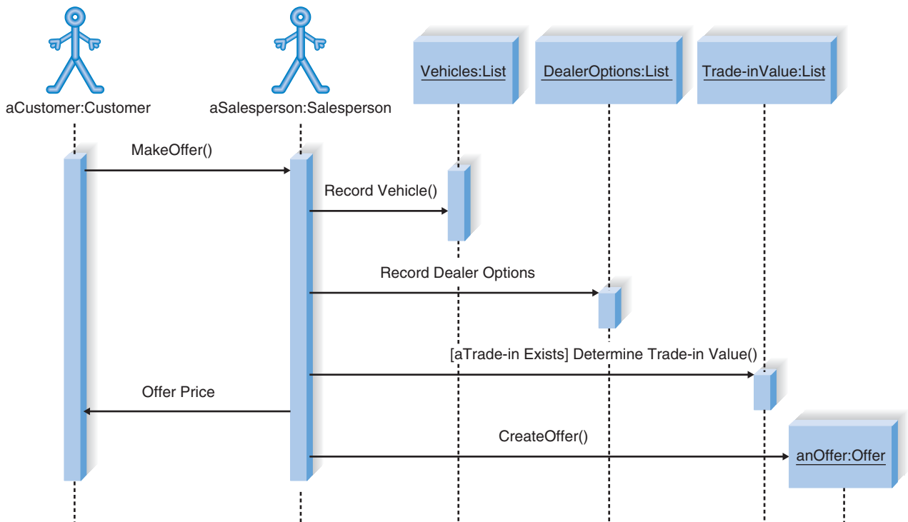
FIGURE 14-21 Sequence Diagram
