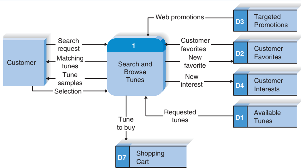
(a) Tune Source Process 1 DFD Fragment
