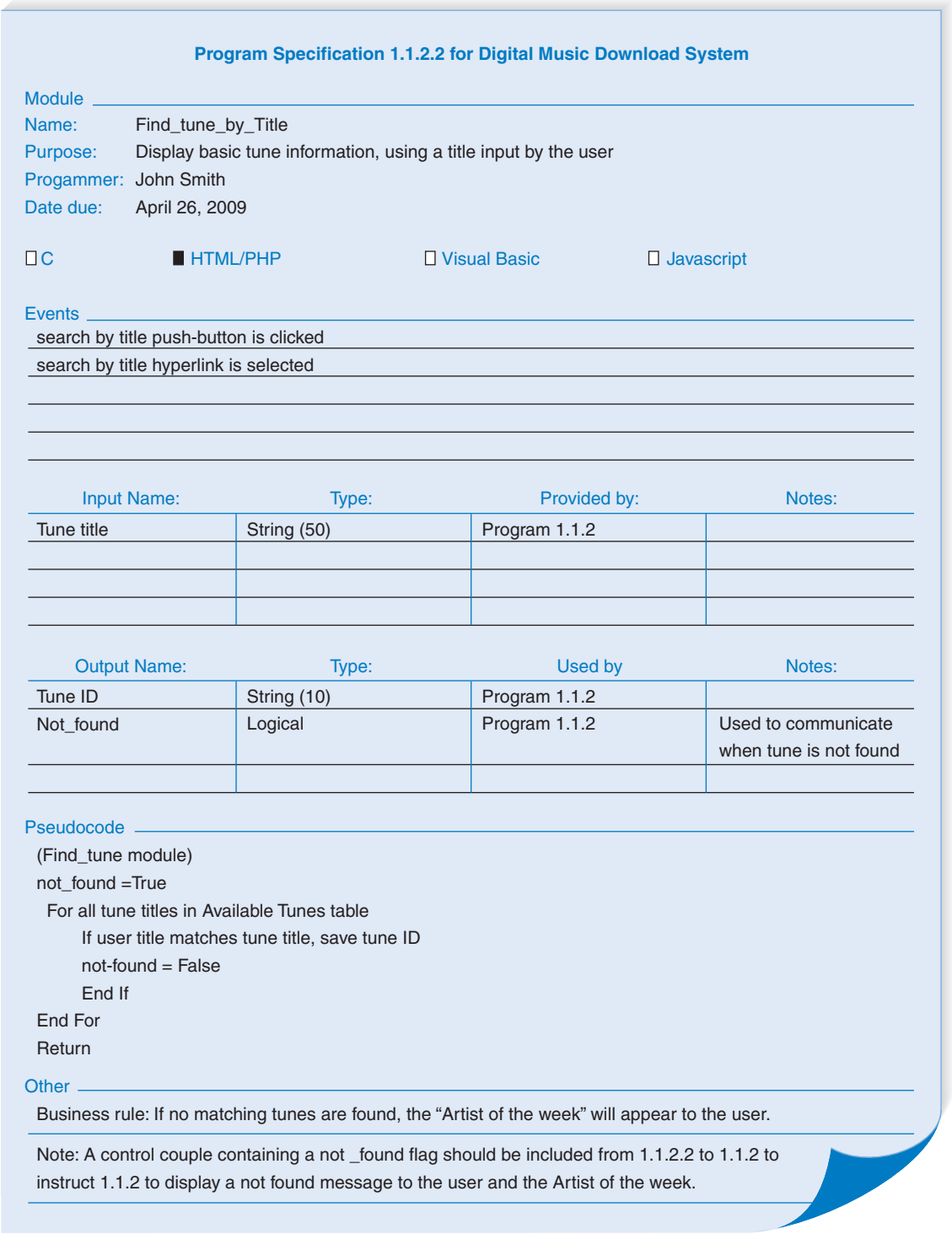
FIGURE 10-22 Program Specification for Find Tune by Title
