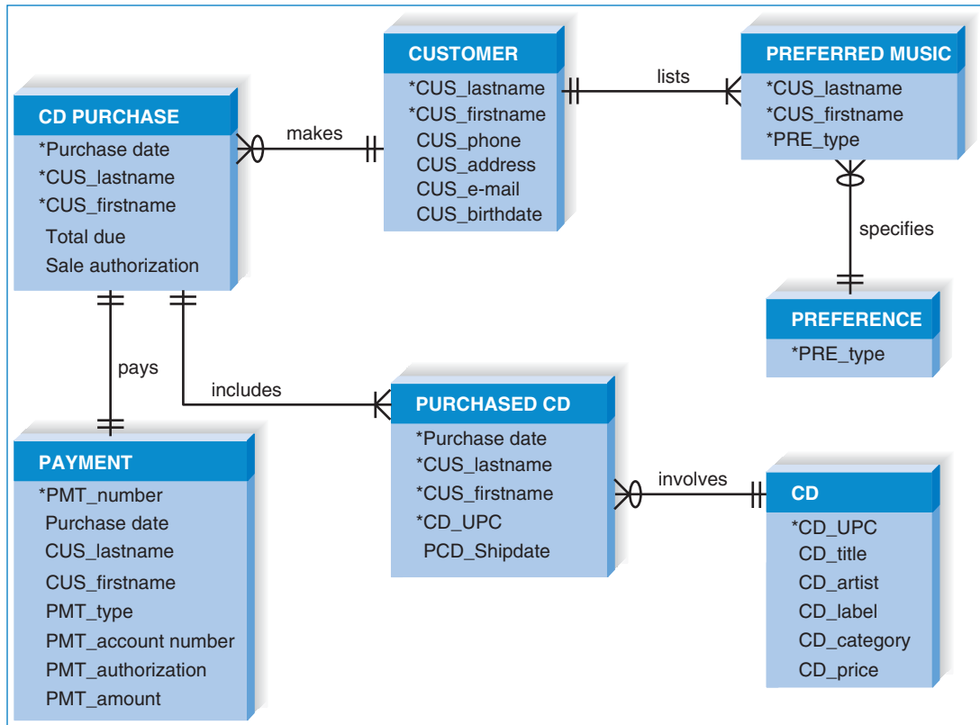
FIGURE 6A-5 Third Normal Form
