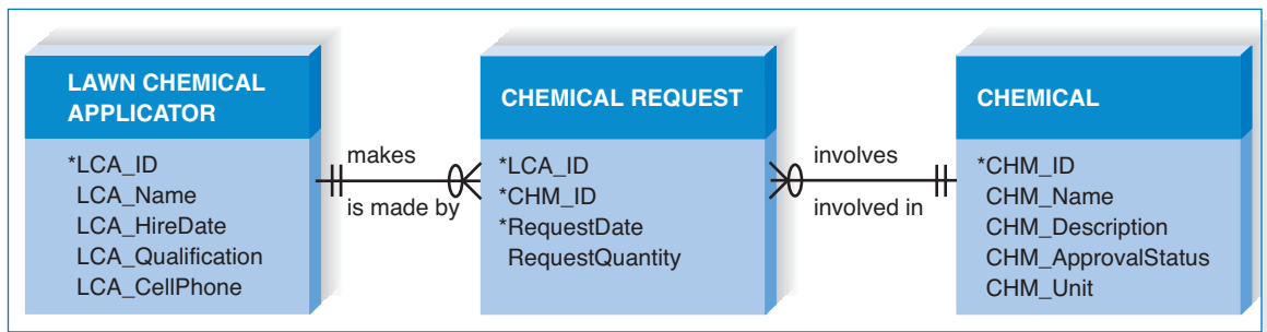
FIGURE 6-1 Chemical Request ERD
