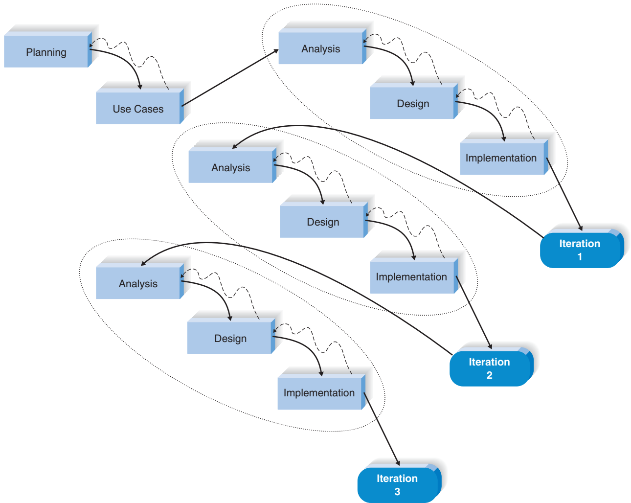
FIGURE 14-8 An Adaptation of the Unified Process Phased Development Methodology
