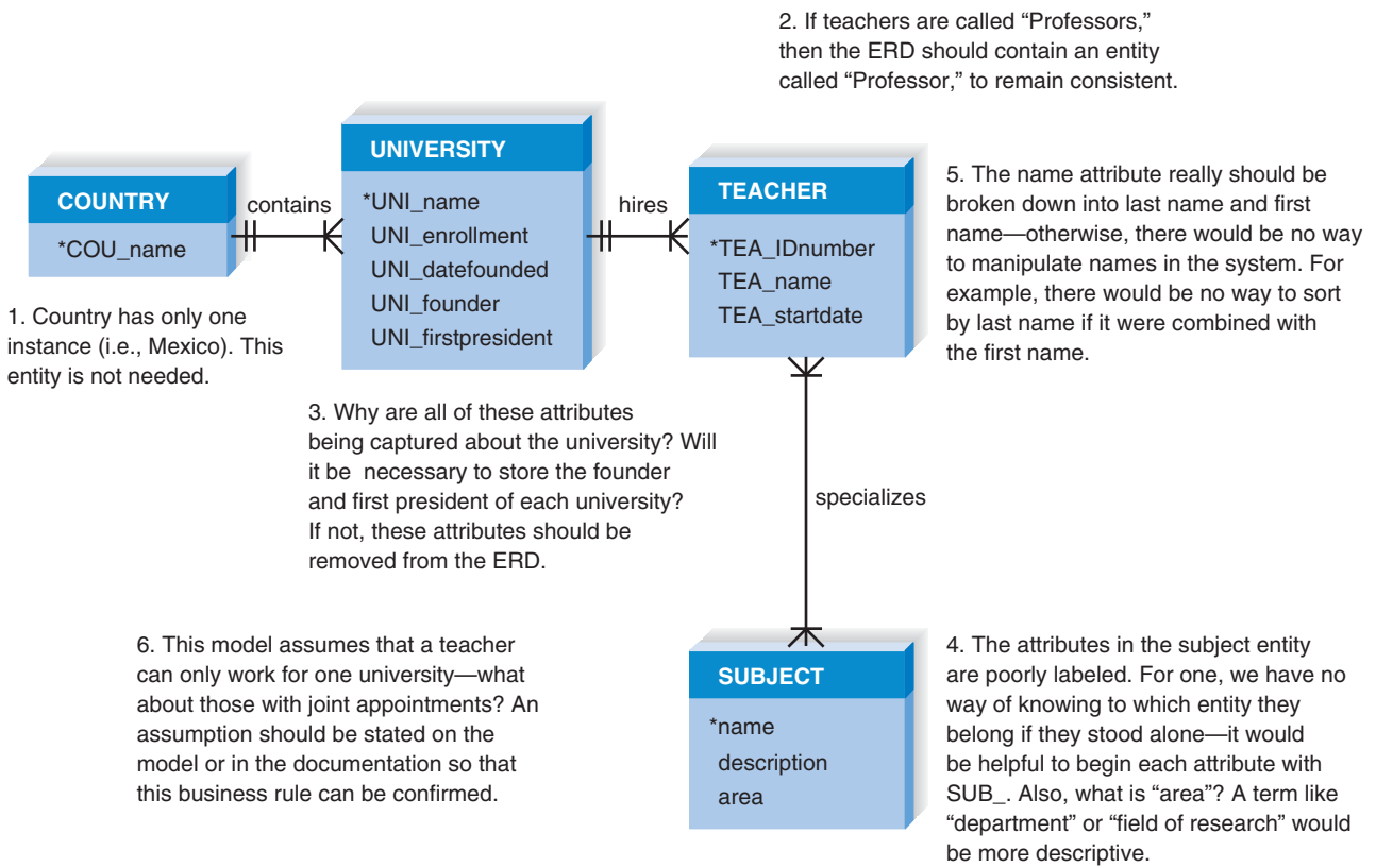
FIGURE 6-15 Data Modeling Guidelines Summary
